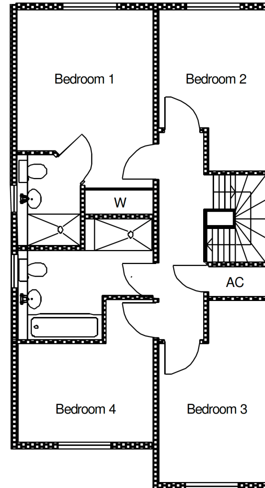
First Floor Layout
